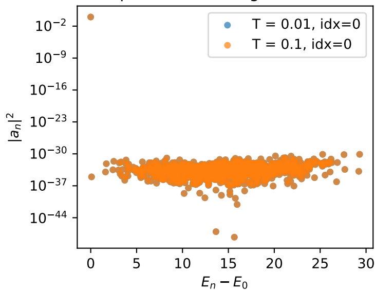
Amplituder vs energi (tid idx=0)
